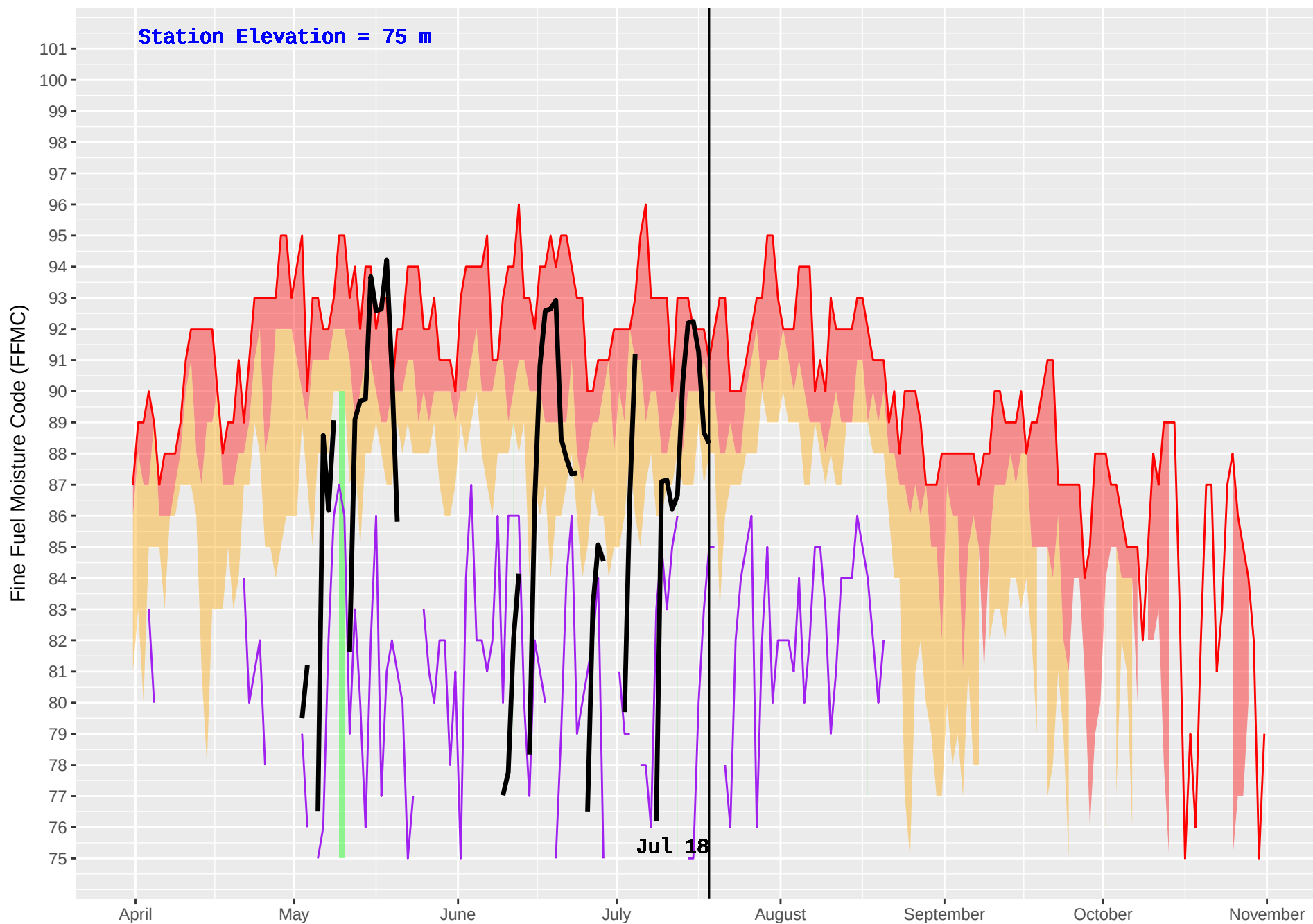
KITPARK (106) : Historical (1995–2016) and Current (2018) Daily Fine Fuel Moisture Code (FFMC)
