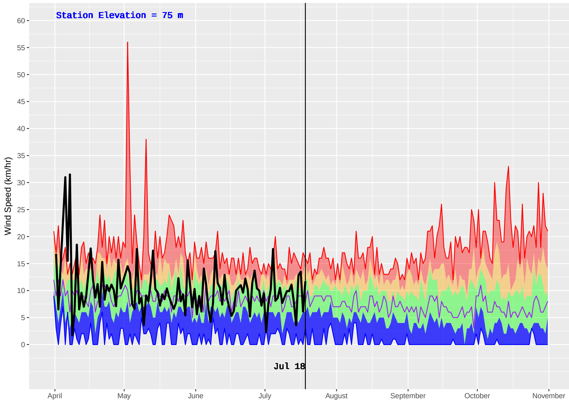
KITPARK (106) : Historical (1995–2016) and Current (2018) Daily Wind Speed
