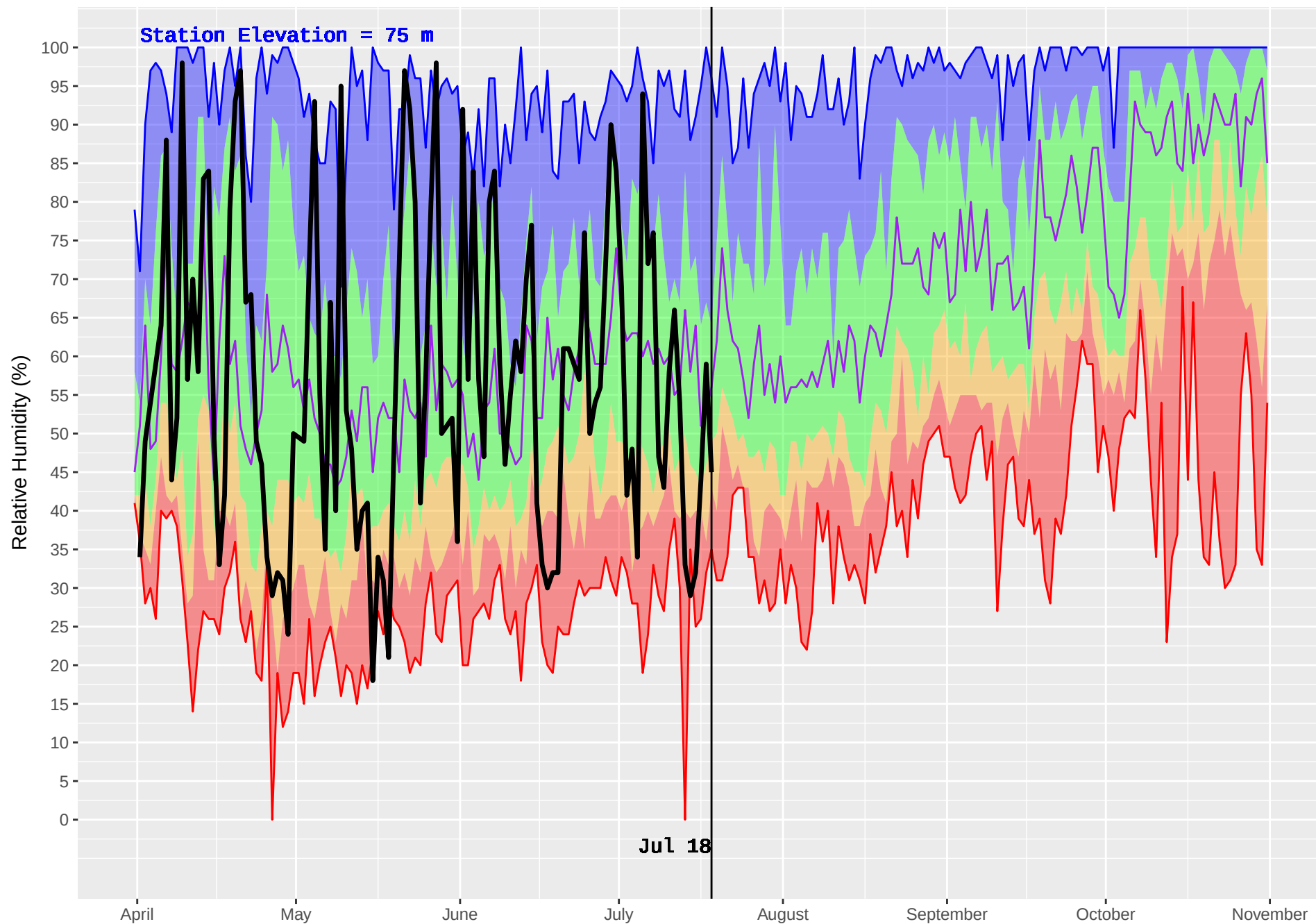
KITPARK (106) : Historical (1995–2016) and Current (2018) Daily Relative Humidity
